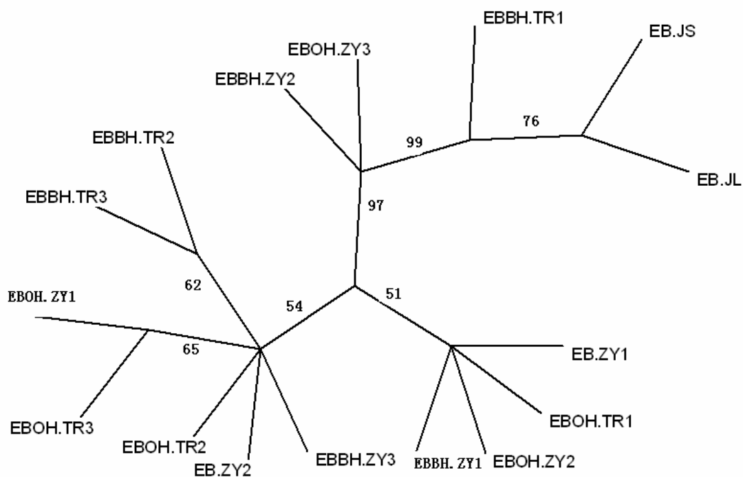
Figure 1: Bootstrap 50% majority-rule consensus tree of two Most Parsimonious Trees Reconstructed on the Basis of ITS Sequence from Fructus Evodiae. Tree length = 153, with a Consistency index (CI) = 0.9673, Homoplasy index (HI) = 0.0327, CI excluding uninformative characters = 0.9231, HI excluding uninformative characters = 0.0769, Retention index (RI) = 0.9664 and Rescaled consistency index (RC) = 0.9349. Number on line is the bootstrap value with 1000 replicates.
