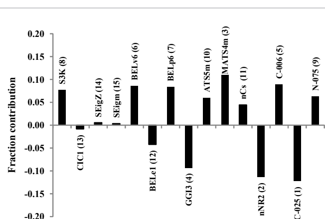
Figure 3: Plot of fraction contribution of MLR-like PLS coefficients (normalized) against 15 identified descriptors (Table 3) associated with MMP-13 inhibition activity of the compounds.
