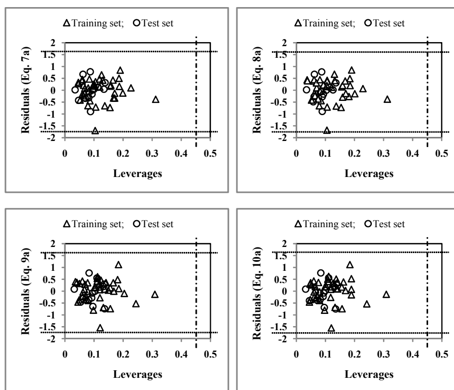
Figure 4: Williams plot for the training-set and test- set for inhibition activity of MMP-13 for the compounds in Chart 1. The horizontal dotted line refers to the residual limit ( \pm 3 \times \text{standard deviation} ) and the vertical dotted line represents threshold leverage h^* ( = 0.439 ).
