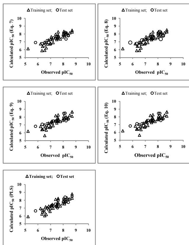
Figure 2: Plot of observed versus calculated pIC_{50} values for training- and test-set compounds.
