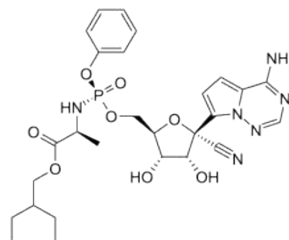
Figure 1: Structure of remdesivir.
