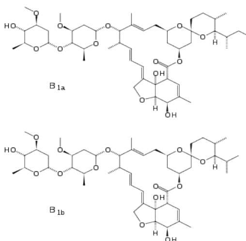
Figure 5: Structure of ivermectin.
