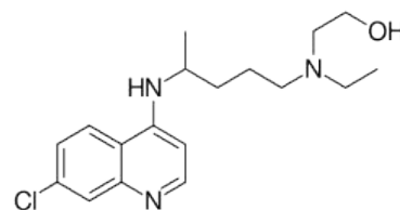
Figure 2: Structure of hydroxychloroquine.
