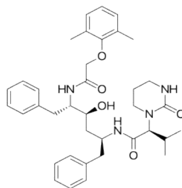
Figure 3: lopinavir.
