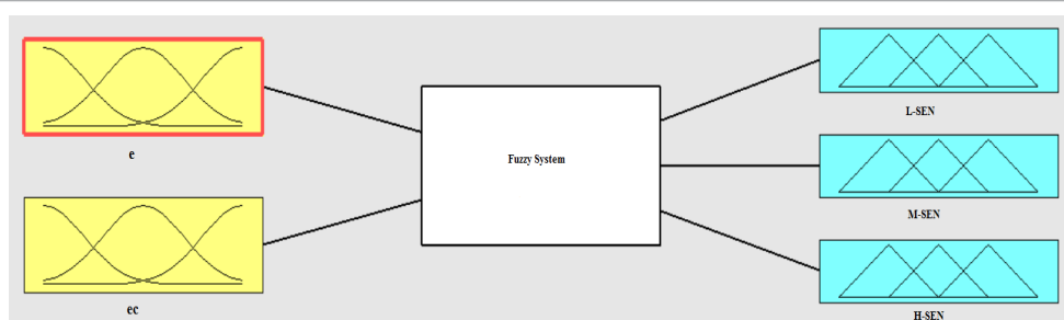
Figure 8: Fuzzy inference system design.
