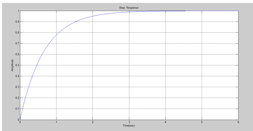
Figure 9: Transient analysis.
