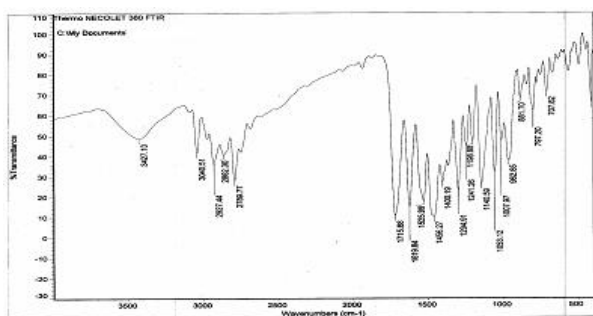
Figure 2 IR Spectra of Aceclofenac
