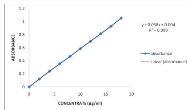
Figure 1 Standard Curve of Aceclofenac
