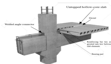
Figure 2: Slab to beam connection.
