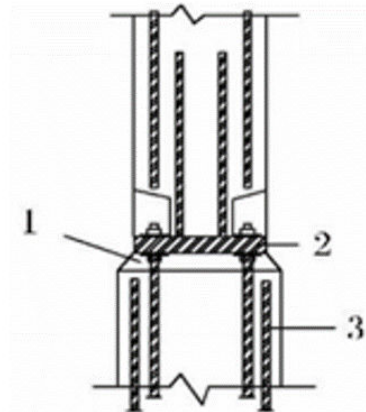
1-Pouring concrete; 2-Steel plate; 3-Inserting steel bar
