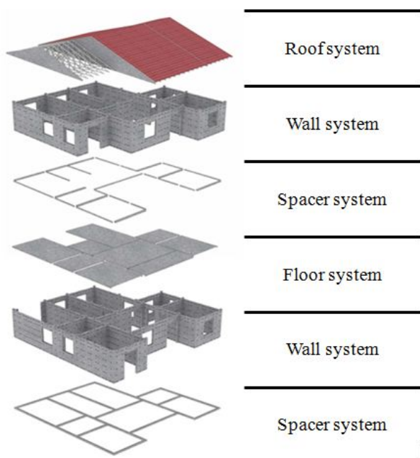
Figure 5: BPC structure.
