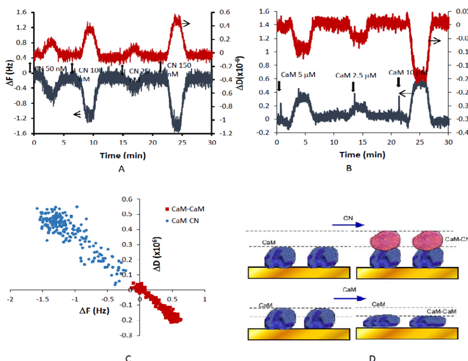
Figure 3: A. Change in frequency ( \Delta F : Deep blue) and dissipation ( \Delta D : Red) of various concentration of calcineurin (CN) binding to immobilized CaM in presence of \text{Ca}^{2+} . This is a typical binding data with negative frequency change and positive dissipation change which indicate increased adlayer due to binding. B. The QCM-D data for CaM dimerization. CaM dimerization also causes positive \Delta F (Deep blue) and negative \Delta D (Red), indicating dimerization causes collapsed structure. C. \Delta D vs. \Delta F plot for CaM dimerization (round markers) compared to a typical binding of CaM-CN (square markers). D. Schematic diagram of CaM-CN and CaM-CaM binding. The average thickness of hydrated protein layers were observed in the QCM-D measurement. The schematics do not represent actual shapes of the proteins.
