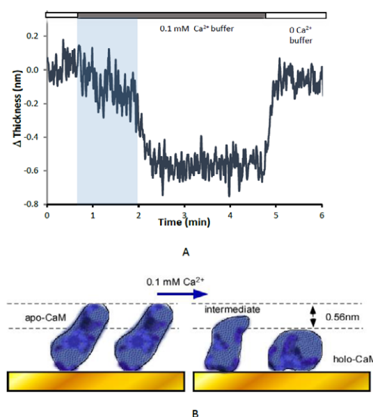
Figure 2: A. The calculated thickness change when the CaM layer is exposed to saturating concentration (0.1 mM) of a \text{Ca}^{2+} buffer. A stable baseline was established at least for 10 minutes prior to \text{Ca}^{2+} application (truncated in the figure). Negative thickness change indicates significant conformation change and molecularly packed structure. The shadowed region shows the initial slow thickness change due to formation of intermediates. B. Schematic diagram to show CaM conformational change with \text{Ca}^{2+} binding. The observed is the average thickness of hydrated CaM or \text{Ca}^{2+} /CaM layer and the schematics do not represent the actual shapes of CaM molecules.
