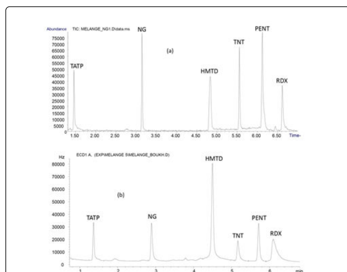
Figure 4: Chromatogram of explosives mixture in acetone obtained by (a) GC/MS (b) GC/ \mu ECD.
