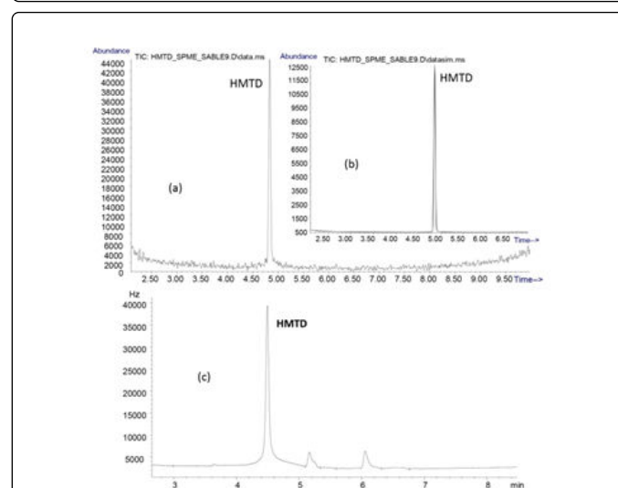
Figure 6: Analysis of HMTD traces in soil (3 mg /150 g) (a) HS-SPME-GC/MS chromatogram with SCAN mode (b) chromatogram with SIM mode (c) HS-SPME-GC/ \mu ECD chromatogram. Stabilization time of glass container (750 mL): 1 h, desorption time in injector: 5 min at 150°C.
