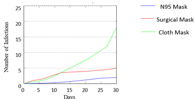
Figure 4: Cumulative infections over 30 days for different masks.
