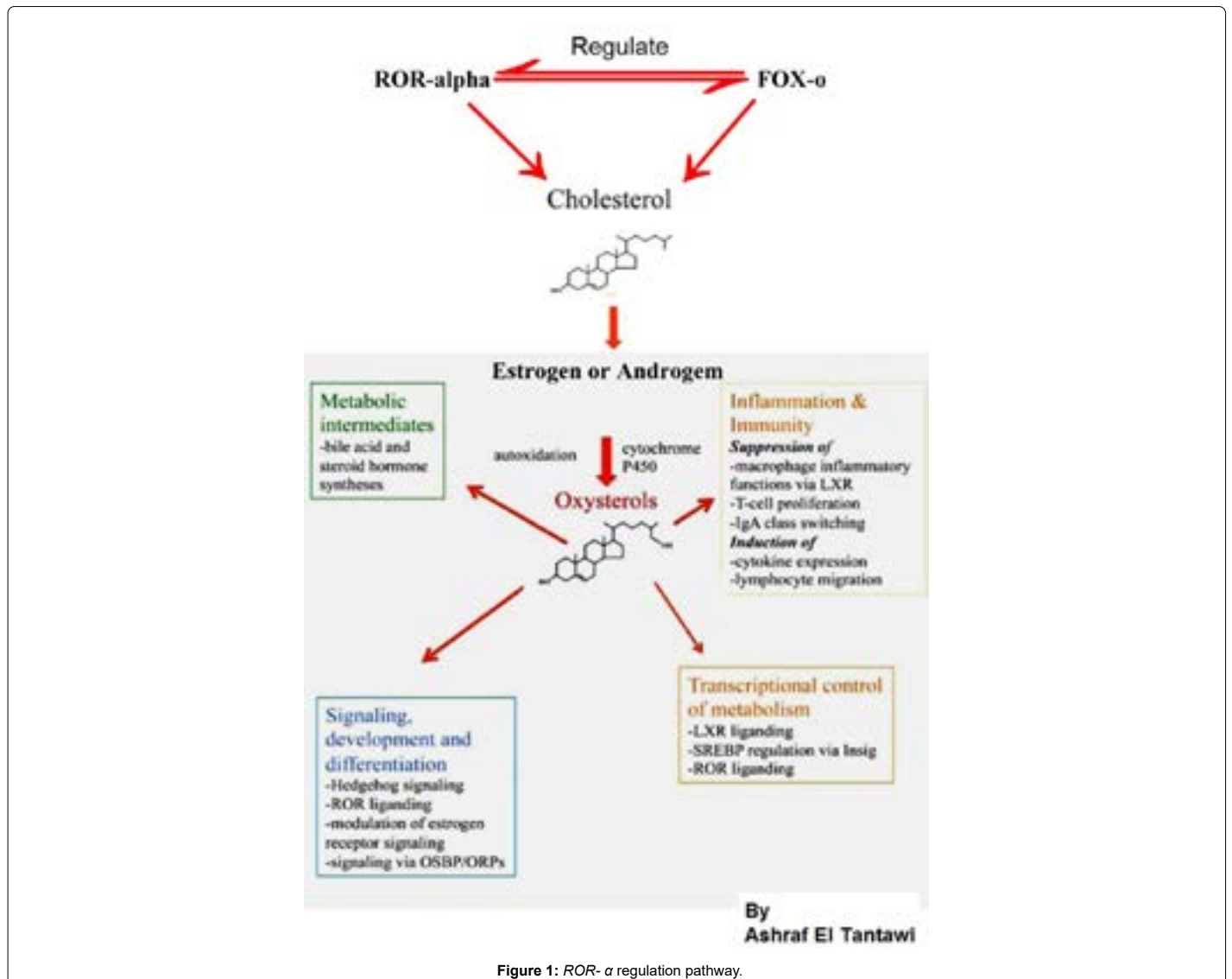
Figure 1: ROR- \alpha regulation pathway.
