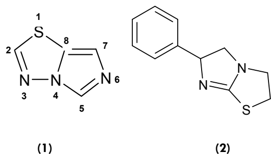
Figure: Imidazole[2,1- b ][1,3,4]-thiadiazole (1) and Levamisole (2)
