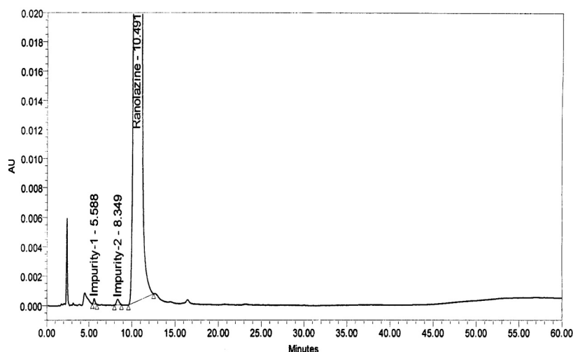
Figure 3: Related Substances Chromatogram of Ranolazine +All Excipients (RZ15) stored at 40°C/75%RH (after 28 days).
