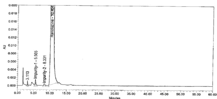
Figure 6: Related Substances Chromatogram of Ranolazine extended release tablets Stored at 40°C/75% RH (after 3 months).
