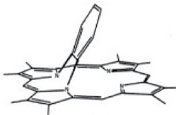
Figure 2: Heme adduct formed by reaction of the heme of cytochrome P450 with autocatalytically activated 1-ABT. The peripheral substituents on the porphyrin are only shown schematically, as isomeric structures that differ in the pattern of peripheral substitution are possible.
