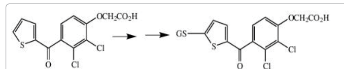
Figure 11: The cytochrome P450-catalyzed transformation of tienilic acid to a glutathione conjugate is inhibited by 1-ABT.
