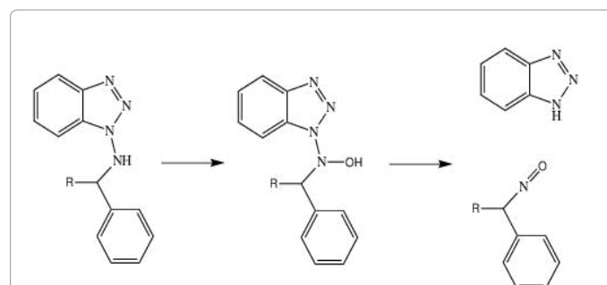
Figure 7: A possible mechanism for the formation of a nitroso compound that could coordinate to the heme iron of P450, resulting in observation of MI complexes. The reaction scheme shown is a modified version of that proposed by Sinal and Bend [90]. The R stands for H, Me, or Et, depending on whether it refers to experiments with compound 13 , 14 , or 15 (Table 2), respectively.
