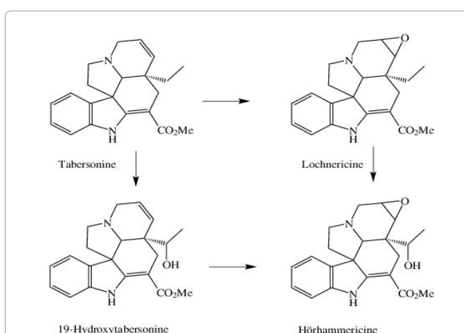
Figure 18: Pathways for the biosynthesis of hürhammericine from tabersonine in the biogenesis of vindoline.
