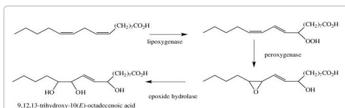
Figure 17: Formation of 9,12,13-trihydroxy-10( E )-octadecenoic acid in Solanum lipoersicum (tomato).
