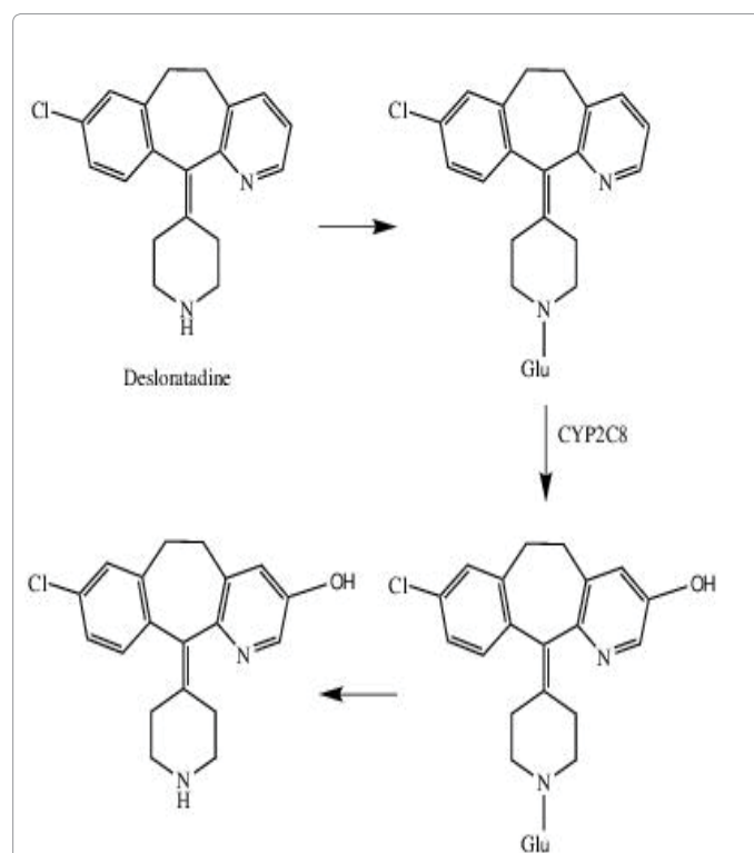
Figure 12: The hepatic metabolism of desloratadine elucidated with the help of 1-ABT.
