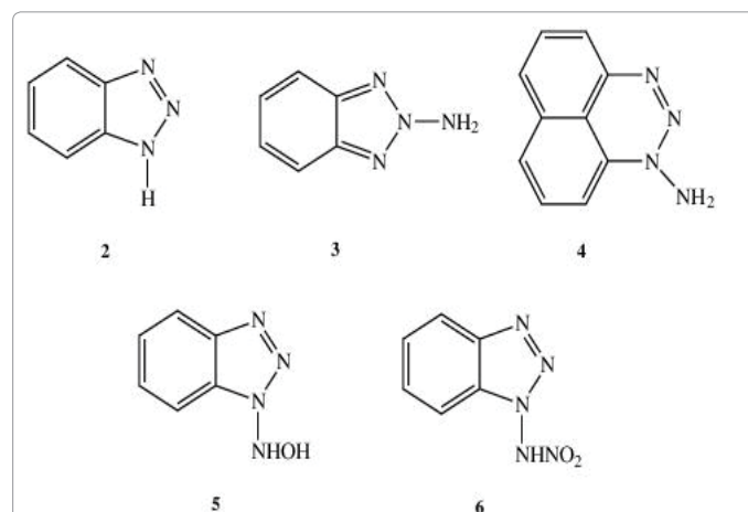
Figure 6: Analogues of 1-ABT with variants of the core 1-aminobenzotriazole structure are not effective mechanism-based inactivating agents.
