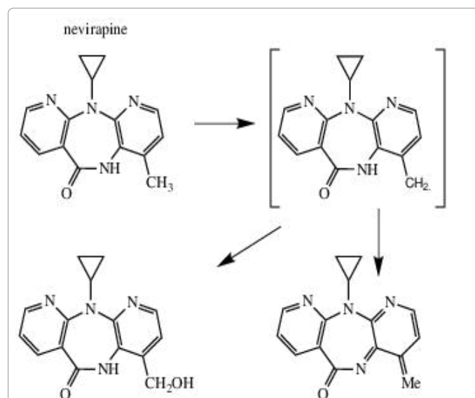
Figure 10: Metabolites of nevirapine formed by cytochrome P450 enzymes.
