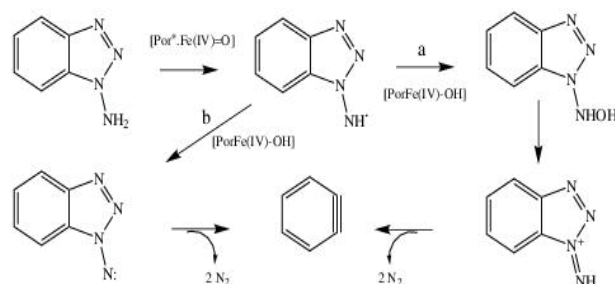
Figure 3: Two possible mechanisms for the P450-catalyzed oxidation of 1-ABT to benzyne, where [\text{Por}^+ \text{Fe(IV)=O}] stands for the activated iron oxo species of cytochrome P450.
