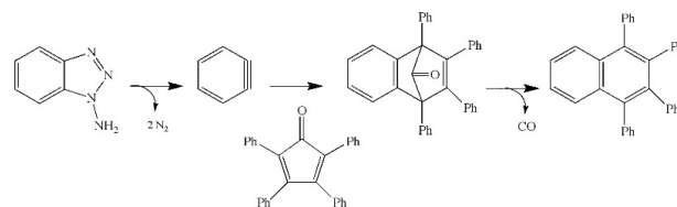
Figure 1: Oxidation of 1-ABT (compound 1) produces benzyne, which can be chemically trapped to give 1,2,3,4-tetraphenylnaphthalene.
