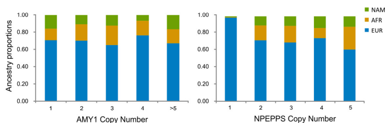
Figure 1: Ancestry proportion estimates differentiated by copy number variation of the AMY1 and NPEPPS genes in 96 individuals of the Brazilian population.
