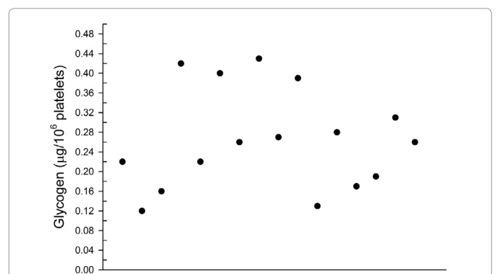
Figure 2: Scatter plot representing the values of glycogen obtained in the PC samples. The figure depicts the values of glycogen ( \mu\text{g} ) from 16 healthy donors, normalized by the number of cells ( 10^6 platelets).
