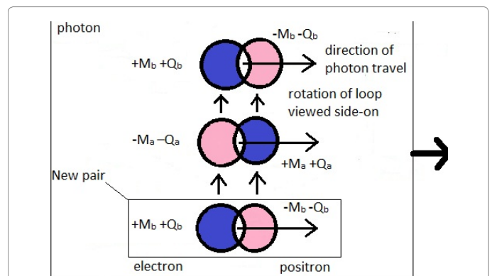
Figure 3: Photon as partially merged electron and positron loop showing chase forces around the loops and between meons in each loop (loop rotational axis in plane of paper). Each new pair is like an original ZMBH but in motion with in the loops.
