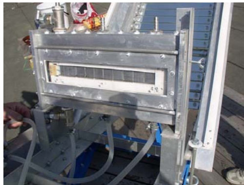
Fig. 11: Experimental PVT receiver in concentrator
