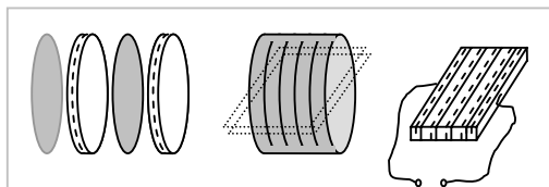
Fig 9: The main steps of fabricating solar cells with vertical p-n-junctions (assembling of wafers with p-n-junctions and aluminum or/and silumin inter-layers foils in stack – on the left, soldered stack with showed cut planes – in the center, vertical p-n-junctions solar cells with external contacts – on the right).
