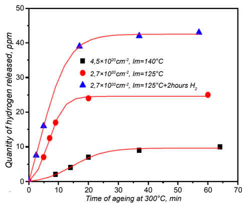
Figure 2: Hydrogen degasation kinetics for irradiated and irradiated+hydrogenated steel.
