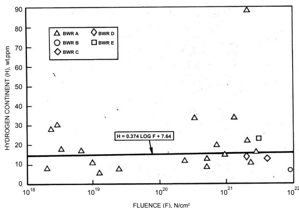
Figure 3. IPH content in 304 SS versus FNF ( E>1\text{ MeV} ).
