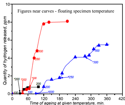
Figure 1: IPH degasation kinetics for irradiated steel ( 4,5 \times 1020\text{cm}^2 at 140^\circ\text{C} ).
