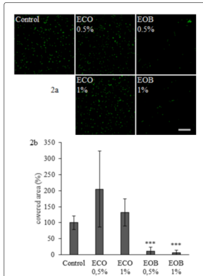
Figure 2: Fluorescence microscopic visualisation of PAO1 attached cells in different conditions (2a) and corresponding relative recovery percentage (2b). Cell adhesion was carried out in control condition, in presence of 0.5% to 1% ECO or in presence of 0.5% to 1% EOB emulsified with 0.5% to 1% ECO. Attached cells were observed with CLSM after SYTO9 staining at magnification x630 and scale represents 67.3 \mu m. Fractions of the covered area obtained with the IMAGEJ software are presented in figure 2b. Error bars represent standard deviation from the mean (n=6) and ***P<0.001.
