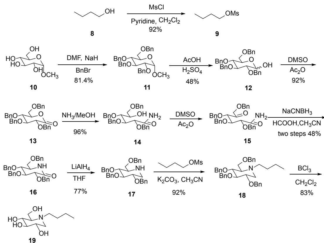
Scheme 1: The improved synthetic route of N -butyl-1-deoxyojirimycin.
