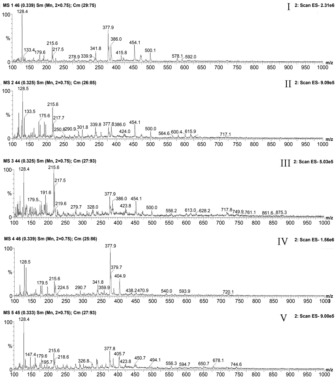
Figure 1: ESI-MS fingerprints of ethanol extracts from five Amaranthaceae whole plants from the south of Brazil (I: Alternanthera philoxeroides , II: Alternanthera hirtula , III: Alternanthera praelonga , IV: Froelichia tomentosa , and V: Pfaffia tuberosa ).
