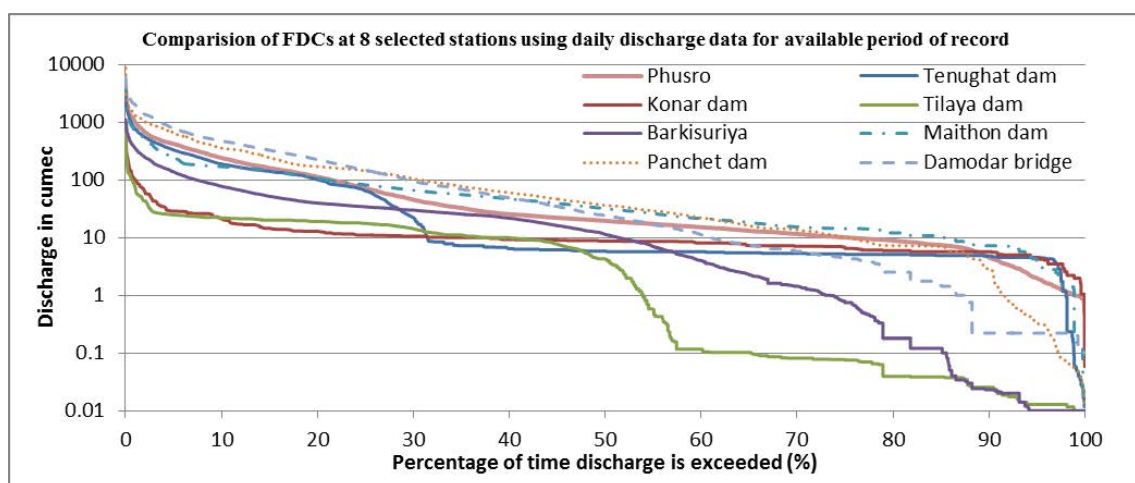
Figure 3: A graphical comparative representation of daily FDC for selected stations in the DRB.
