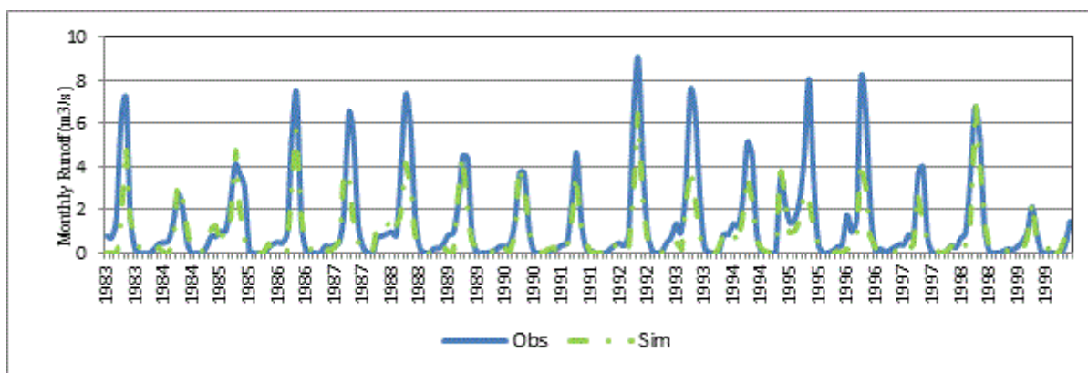
Figure 10: Observed and modelled stream flow for the calibration period (1983-1999).
