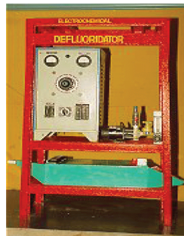
Figure 4: Electrochemical defluoridator.
