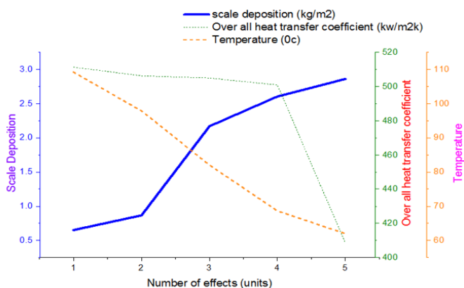
Figure 4: Over all heat transfer coefficient and temperature profile with respect to scale deposition in MEE.
