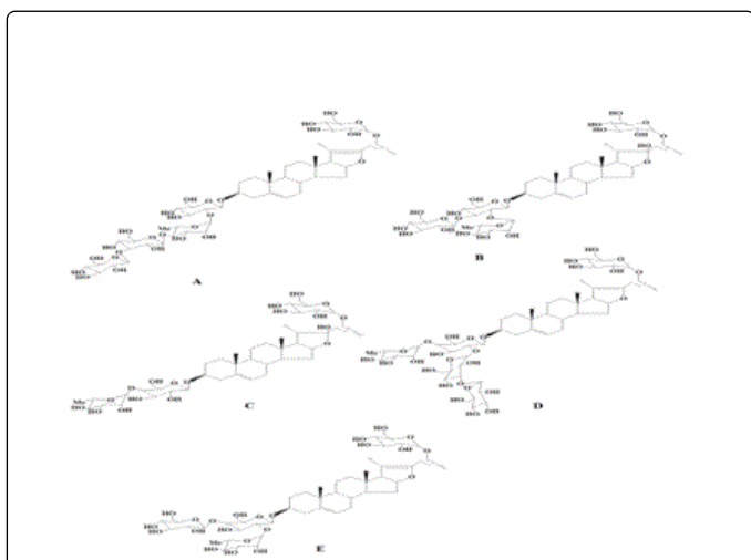
Figure 4: Chemical structures of compounds from Dioscorea zingiberensis C.H.Wright. (A): Compound A; (B): Compound B; (C): Compound C; (D): Compound D; (E): Compound E.
