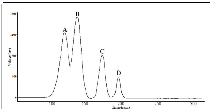
Figure 1: CCC chromatogram of total steroid saponins. Solvent system: ethyl acetate-n-butanol-methanol-water (4:1:2:4, v/v); stationary phase: upper organic phase; mobile phase: lower aqueous phase; flow-rate: 2.0 ml min -1 ; revolution speed: 850 rpm; sample: 100 mg dissolved in 10 ml lower phase; retention of the stationary phase: 42%; Alltech 800 ELSD condition: drift tube temperature: 55°C; gas flow rate 3.0 L min -1 .
