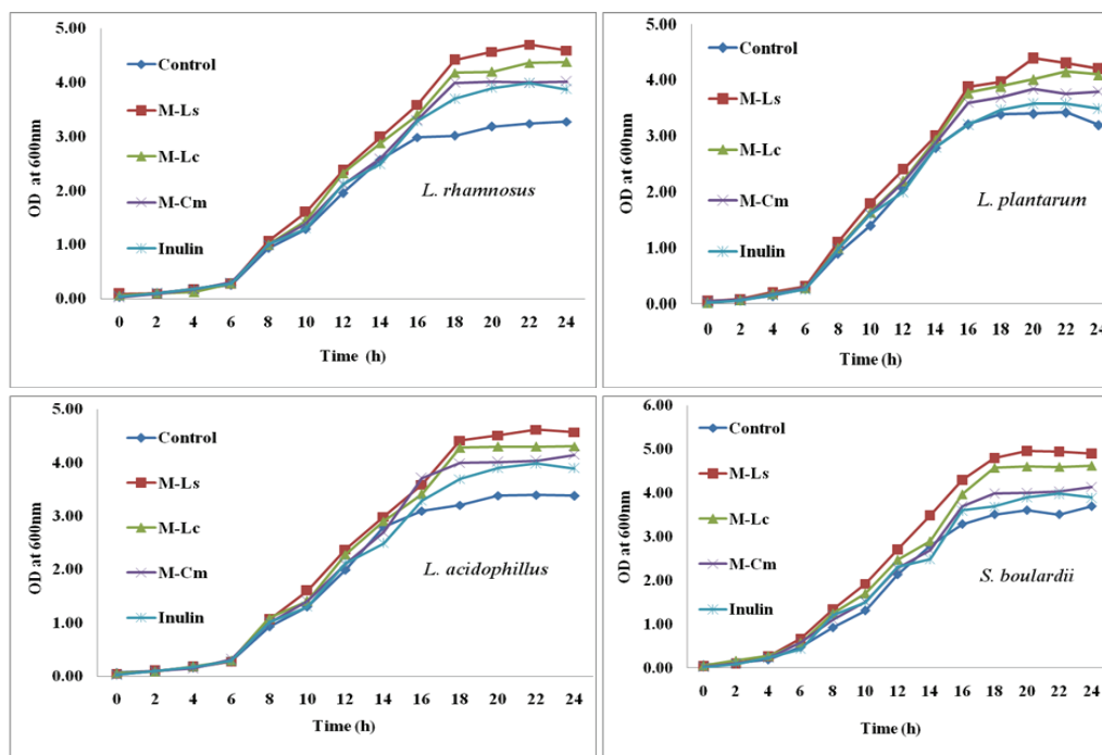
Figure 1: Strains of Lactobacilli and S. boulardii were grown on MRS and YEPD growth medium and optical density was read at the intervals of 2 h for 24 h.
