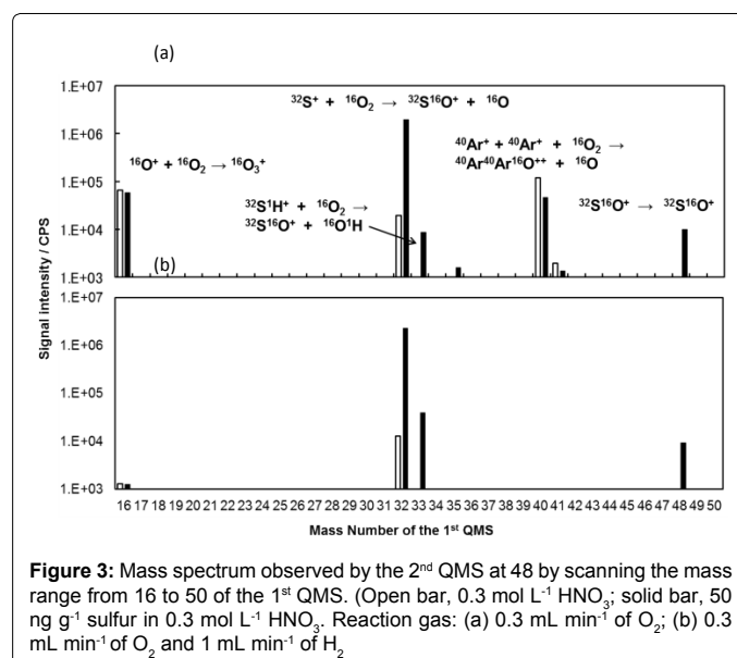
Figure 2: The mechanism of ICP-QMS/QMS for removing spectral interferences.
