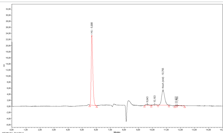
Figure 1: Chromatogram of hydroxyurea aqueous solution (10 mg/L) enriched with internal standard.
