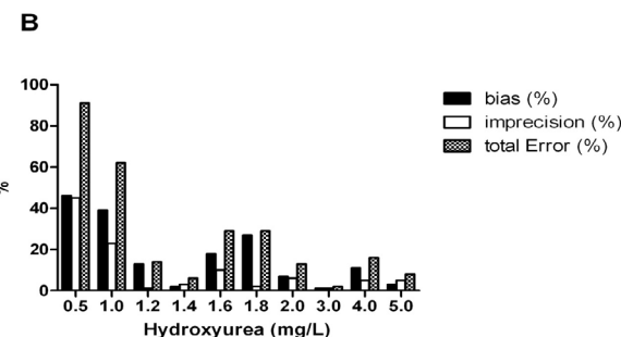
Figure 4: Estimation of the limit of quantification (A) In water (B) In plasma.
