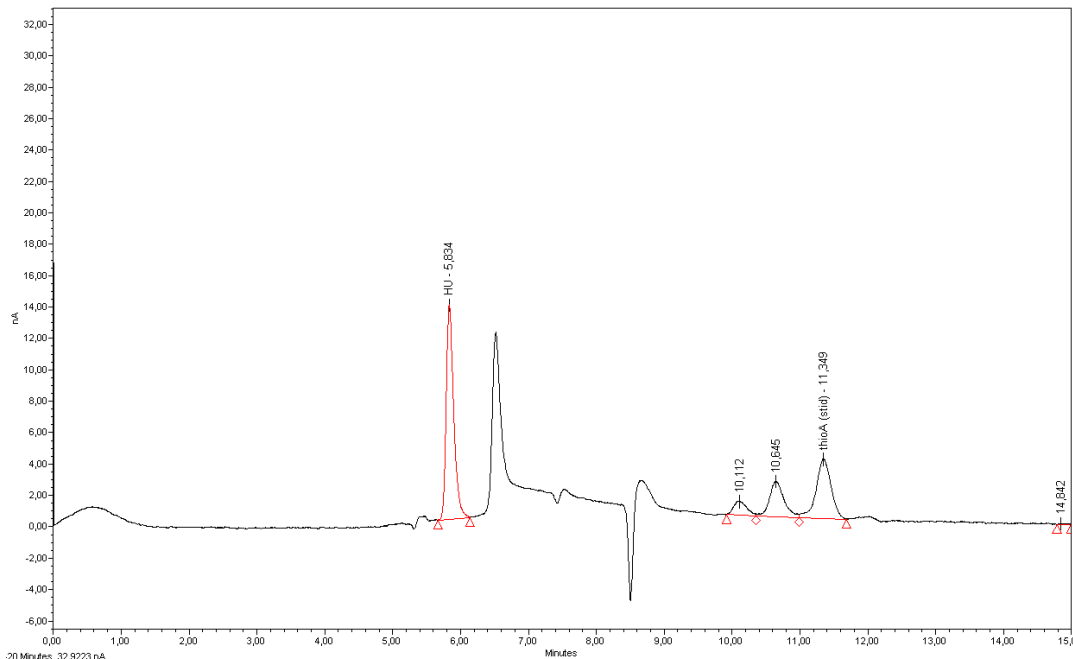
Figure 2: Chromatogram of hydroxyurea plasma solution (10 mg/L) enriched with internal standard.
