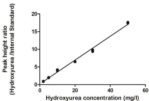
Figure 3: Typical plasma calibration curve.
