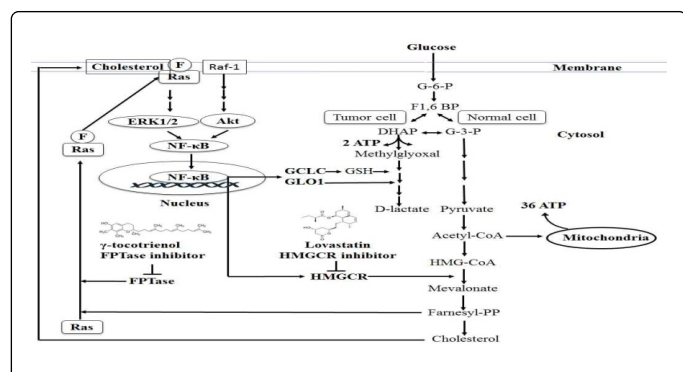
Figure 1: Schematic model of lipid raft-mediated signalling in the regulation of cell survival and apoptosis in cancer cells during cholesterol depletion treatment. This scheme highlights the importance of lipid raft membrane domains for NF- \kappa B constitutive activation in the regulation of cancer cell survival enzymes and the inhibition of cholesterol biosynthesis leading to the disruption of lipid raft and the subsequent apoptosis.
