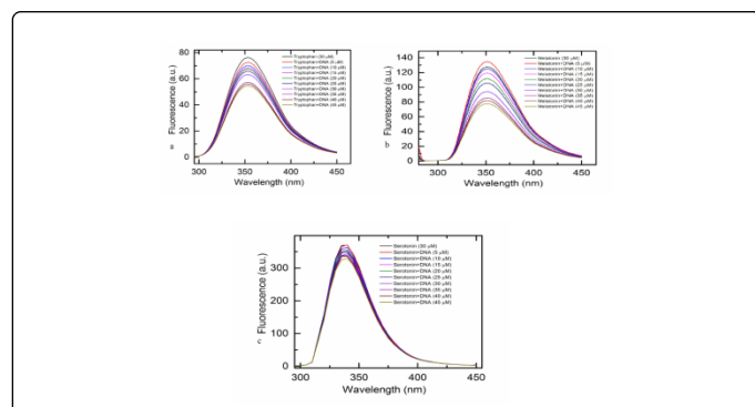
Figure 2: Effect of increasing concentrations of native calf thymus DNA on the fluorescence emission spectra of a) tryptophan, b) melatonin and c) serotonin. The compounds (in 10 mM Tris-HCl, pH 7.5) were excited at 280 nm in the presence of increasing native DNA base pair molar ratios. The emission spectra was recorded between 300-450 nm.
