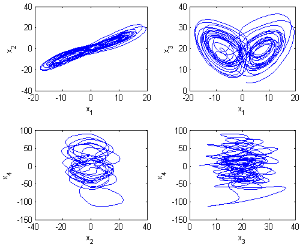
Figure 1: Diagram of the attractors.
