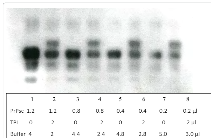
Figure 4: Showed in presence of TPI a reduced immune detectability of the PrPsc bands compared to that of controls. Also in presence of TPI but not in the controls an unexpected immune detected new band having a molecular weight of 33 KD was observed just above the PrPsc upper bi-glycosylated 29 KD band which was markedly reduced about half in volume.
