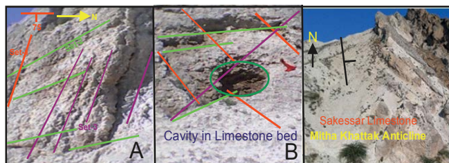
Figure 3: Photographs showing joint system in Sakesar L.s eastern limb of MKA.
