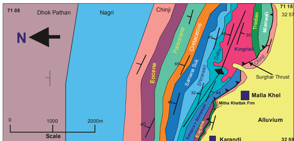
Figure 6: Geological map of the Karandi and Malla Khel areas of Surghar Range.
