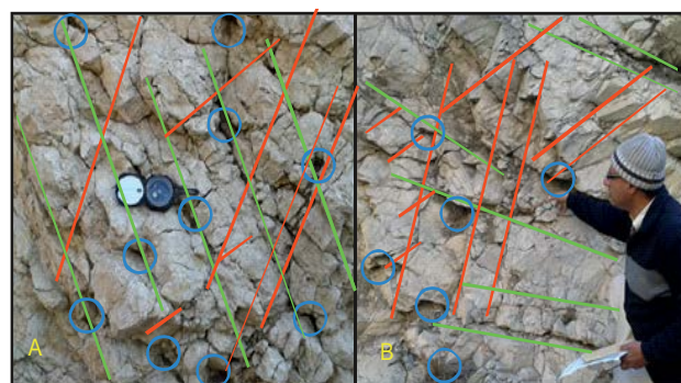
Figure 5: Showing fractured Sakesar Limestone with joints rose diagram of KA.
