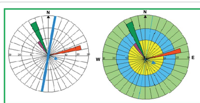
Figure 4: Joints rose diagram along with structural trend data eastern limb of MKA.
