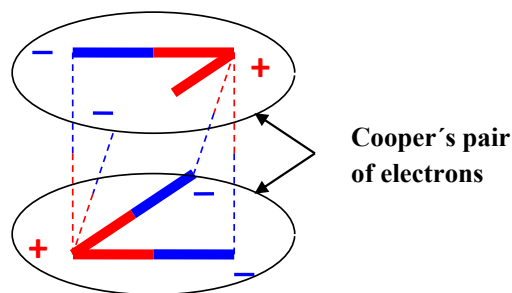
Figure 8: Issutration of Cooper's pair.
