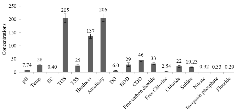
Figure 3: Physico-chemical characteristics of Gomti river water quality during post-idol immersion.
