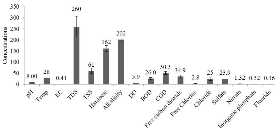
Figure 2: Physico-chemical characteristics of Gomti river water quality during idol immersion.
