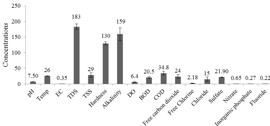
Figure 1: Physico-chemical characteristics of Gomti river water quality during pre-idol immersion.
