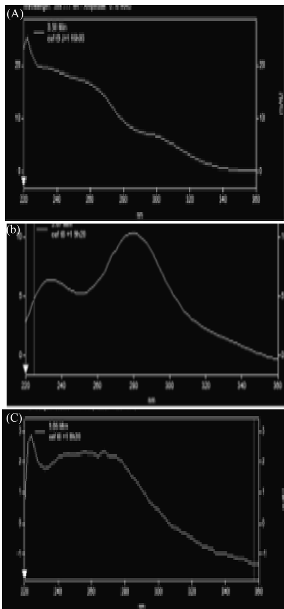
Figure 4: UV spectra of degradation products obtained: (a), (b) and (c) spectrum corresponding to peak 1, 2 and 3 on chromatogram.
