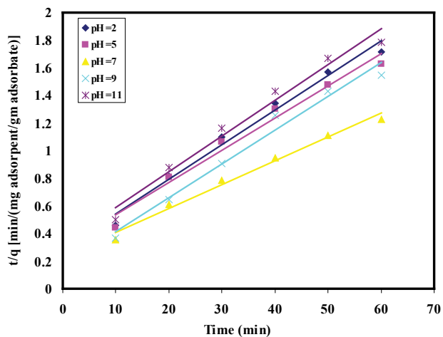
Figure 6: Pseudo second-order equation at different pH values at dye concentration 50 mg/l, 25°C, and 1 gm/l adsorbent dose.
