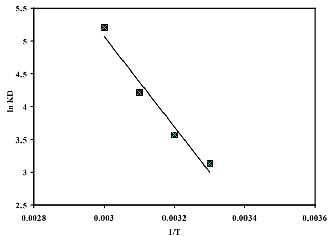
Figure 9: Plot of 1/T versus \ln K_D .
