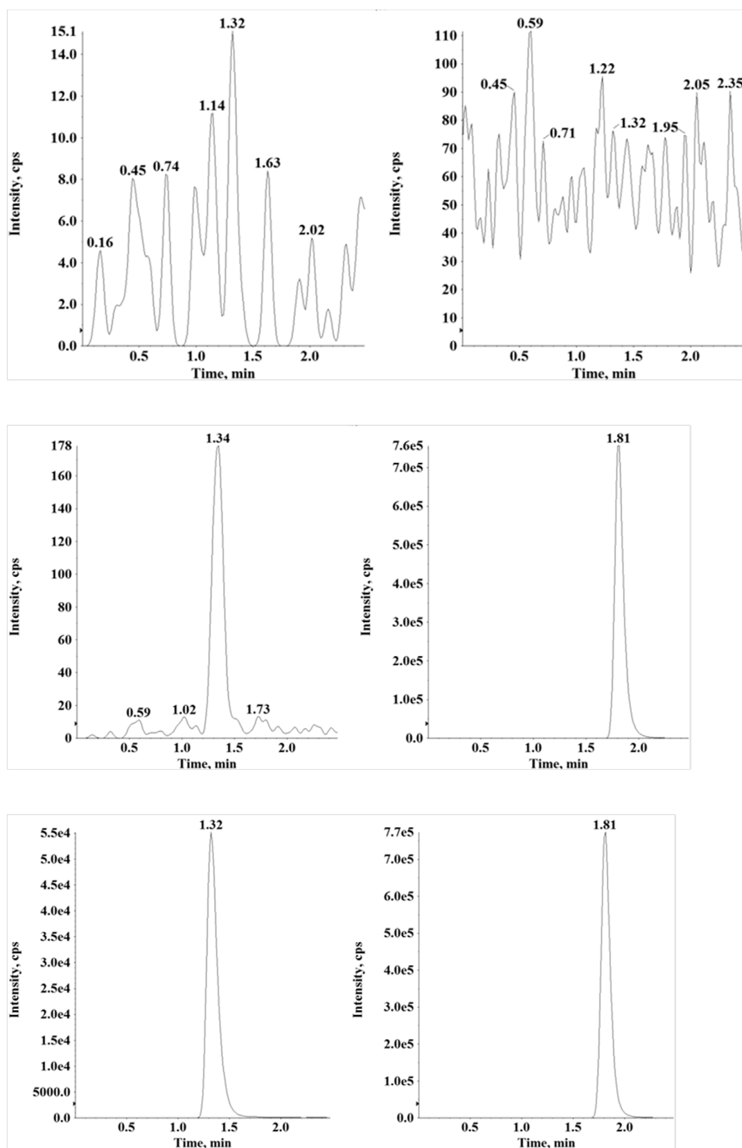
Figure 4: Typical MRM chromatograms of GSK-199 (left panel) and IS (right panel) in (a) mice blank plasma (b) mice blank plasma spiked with GSK-199 at LLOQ (2.52 ng/ml) and IS (c) a 0.25 h in vivo plasma sample showing GSK-199 peak obtained following oral administration to mice along with IS.
