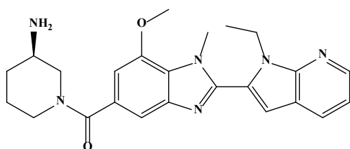
Figure 1: Structural representation of GSK-199.
