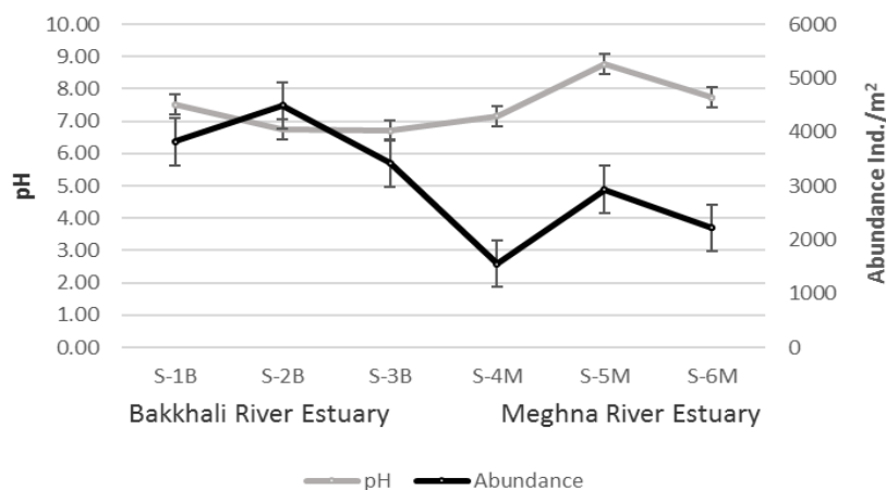
Figure 3: Relationship between the changes of pH and abundance of macro benthic communities in the study sites. Bars indicate Standard Error.
