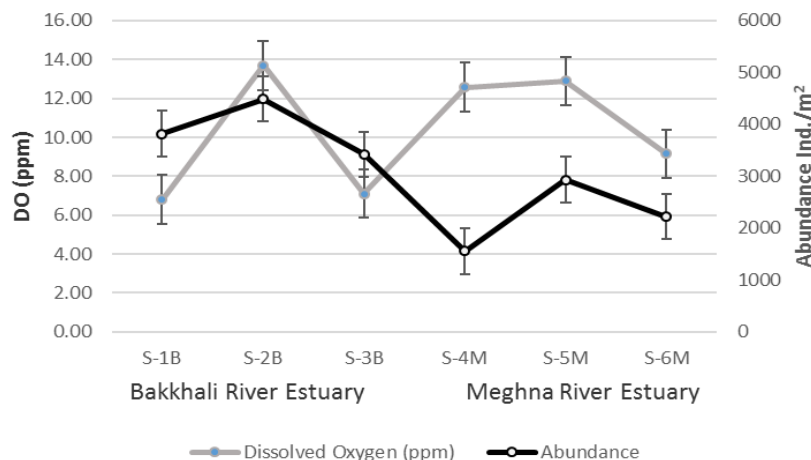
Figure 4: Relationship between the changes of DO (ppm) and abundance of macro benthic communities in the study sites. Bars indicate Standard Error.
