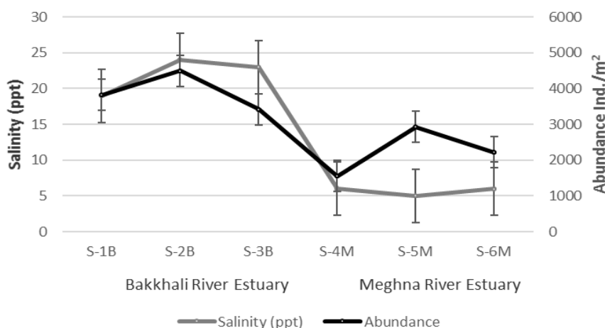
Figure 2: Relationship between the salinity (ppt) and abundance of macro benthic communities observed in the study sites. Bars indicate Standard Error.
