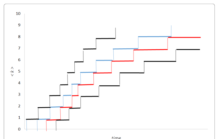
Figure 3: Array of N_0 generation lines with overlap of generation times. Each k -step stair corresponds to the averaged (Figure 2) duplication tree of a generation line (Figure 1). At any time, the system hosts cells belonging to different generation steps.
