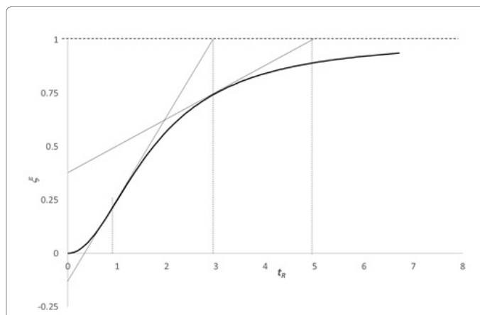
Figure 5: Master plot for the microbial growth. \xi is the fraction of the potential growth actually attained, while t_r is the reduced time, t/t' . The figure includes the tangents at t_r=1 and 3 (namely, t' and t_{end} , respectively) and relevant intercepts.
