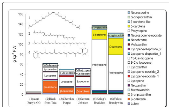
Figure 4: Cumulative carotenoids components (Table 1) of the six American heirloom tomatoes ( Solanum lycopersicum ) studied. Molecular formulas of the main non-oxygenated carotenoids of neurosporene, lycopene, \beta -carotene and \zeta -carotene are indicated. The main metabolic steps (numbers 1 to 4) and molecular formulas from non-cyclic carotenoids of (1) \zeta -carotene \rightarrow (2) prolycopene \rightarrow (3) lycopene to, \rightarrow cyclic carotenoid (4) \beta -carotene are indicated.
