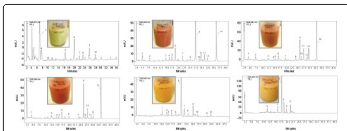
Figure 3: HPLC profiles of carotenoids of the six American heirlooms tomatoes ( Solanum lycopersicum ) studied AR - 'Aunt Ruby's German Green': 1 - Lutein, 2 - Chlorophyllid B, 3 - Chlorophyll B, 4 - Chlorophyll B, 5 - Neoxanthin, 6 - \beta -carotene, 7 - 13-cis-lycopene, 8 - Rubixanthin, 9 - Lycopene, 10 - \gamma -carotene. BF - 'Black from Tula': 1 - Lutein, 2 - Chlorophyll B, 3 - Lycopene diepoxide, 4 - Mutatoxanthin, 5 - Neoxanthin, 6 - cis-neoxanthin, 7 - Lycopene-epoxide 1, 8 - cis- \beta -carotene, 9 - \beta -carotene, 10 - Lycopene, 11 - 13-cis-lycopene, 12 - Rubixanthin, 13 - 9-cis-lycopene, 14 - Lycopene. CP - 'Cherokee Purple': 1 - Lutein, 2 - Chlorophyll B, 3 - Lycopene diepoxide, 4 - Mutatoxanthin, 5 - Neoxanthin, 6 - Cis-neoxanthin, 7 - Lycopene-epoxide 1, 8 - Lycopene, 9 - \beta -carotene, 10 - 15-Cis-lycopene, 11 - 13-Cis-lycopene, 12 - Rubixanthin, 13 - 9-Cis-lycopene, 14 - Lycopene. GJ - 'German Johnson Regular Leaf': 1 - Lutein, 2 - Lycopene diepoxide, 3 - Mutatoxanthin, 4 - Neoxanthin, 5 - Cis-neoxanthin, 6 - Lycopene-epoxide 1, 7 - Lycopene, 8 - \beta -carotene, 9 - 15-Cis-lycopene, 10 - 13-Cis-lycopene, 11 - Rubixanthin, 12 - 9-Cis-lycopene, 13 - Lycopene. KB - 'Kellogg's Breakfast': 1 - Prolycopene epoxide, 2 - Mutatoxanthin, 3 - Neoxanthin, 4 - Cis-neoxanthin, 5 - Neochrome, 6 - Prolycopene, 7 - Proneurosporene, 8 - Violaxanthin, 9 - \beta -carotene, 10 - 13-Cis-lycopene, 11 - 9-Cis-lycopene, 12 - Lycopene; YB - 'Yellow Brandywine Platfoot Strain': 1 - Prolycopene epoxide, 2 - Neochrome, 3 - Prolycopene, 4 - Proneurosporene, 5 - \zeta -carotene, 6 - \alpha -cryptoxanthin; Photos of the meshed fruit saps prepared for HPLC analysis are indicated.
