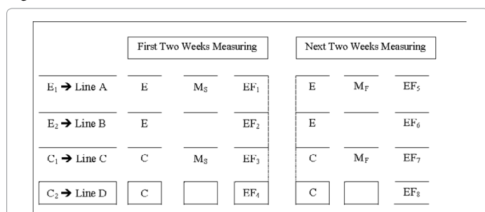
Figure 3: Experimental Design where E denotes the randomized experimental groups (groups are equal except for random differences). C denotes the randomized control groups (groups are similar except for random variations). Subscript indicates the number of groups involved in the study. EF stands for measurement of units produced (efficiency), pretest or posttest. Index indicates efficiency ratio per cluster sampled -cluster is used indifferently as group or assembly line. MS represent the experimental treatment (playing slow music tempo on the manufacturing floor).
