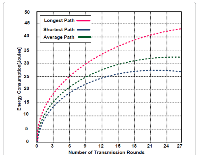
Figure 3: Energy Consumption graph of NLEE Protocol.
