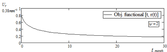
Figure 6: Simulation of dynamic optimal control function, r(t)=0.8 .
