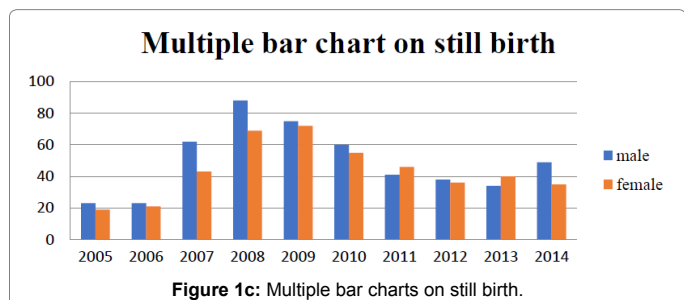
Figure 1c: Multiple bar charts on still birth.
