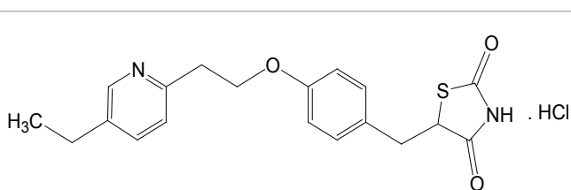
Figure 1: Pioglitazone hydrochloride chemical structure.
