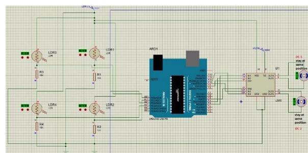
Figure 14: Condition when the entire LDR sensors received the same light intensity.
