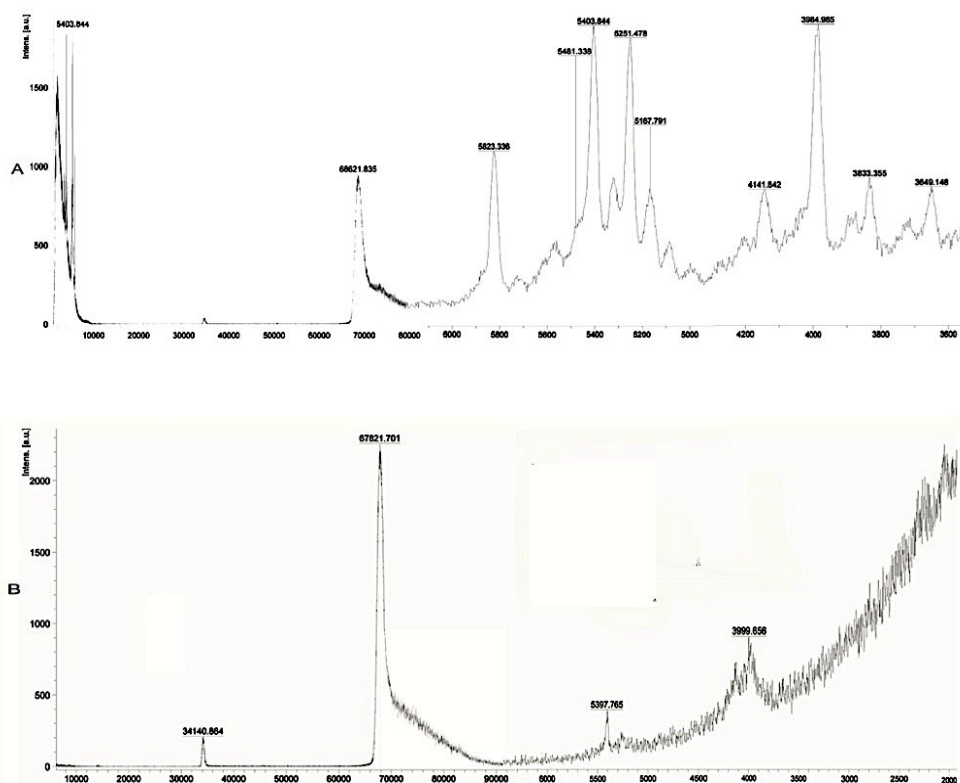
Figure 3: Chromatogram (a) show mono- di- and tri- adducts of BSA+ glucose after incubation 15 days at 37°C. MALDI TOF MS spectra (b) of monomero-glucose, dimero-glucose and trimero-glucose adducts of 2 \alpha ,3 \beta ,21 \beta ,22 \alpha ,29 \alpha -pentahydroxy-olean-12-en-28-oic acid.
