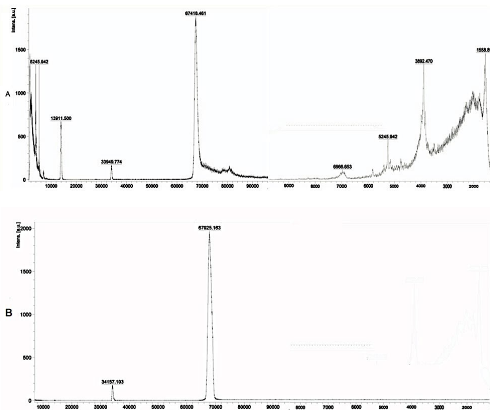
Figure 2: Positive ion MALDI linear TOF MS, with the standard (sinapic acid) SEM detector (a) and BSA (b).
