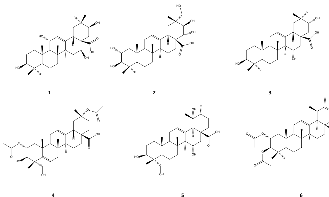
Figure 1: Triterpenoids isolated from Origanum majorana .
