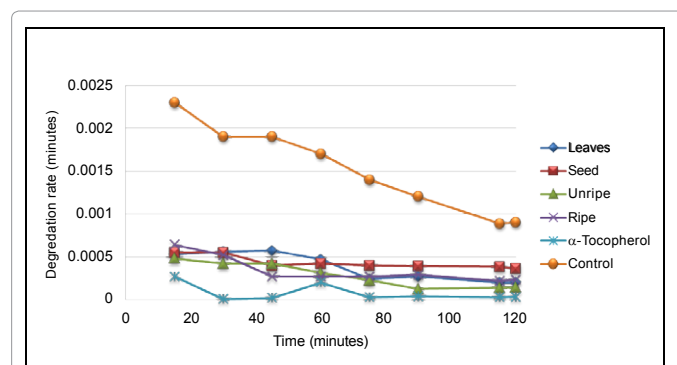
Figure 1: Degradation rates of different parts of CP extracts by b-carotene bleaching method (n=3). Concentration sample was 0.04 mg/ml. Alpha-tocopherol at 200 ppm was used as the standard.
